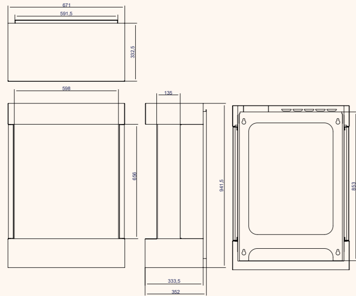
Nebula/Sedona 610 Wall
