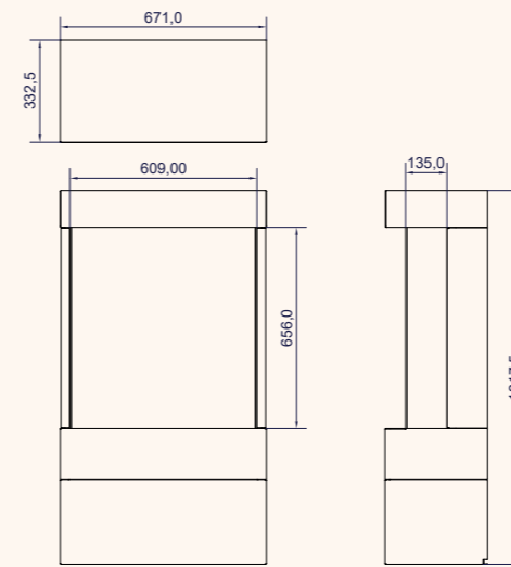
Nebula/Sedona 610 Base
